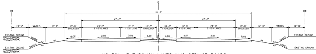
US 301 - 3 THROUGH LANES W/O SERVICE ROADS
