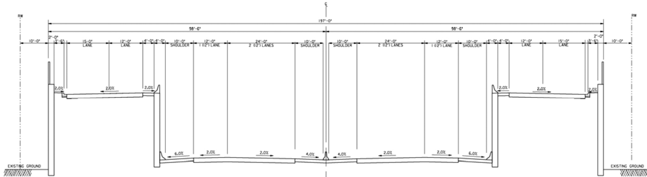
US 301 AT GRADE - 3 THROUGH LANES AT INTERCHANGES
