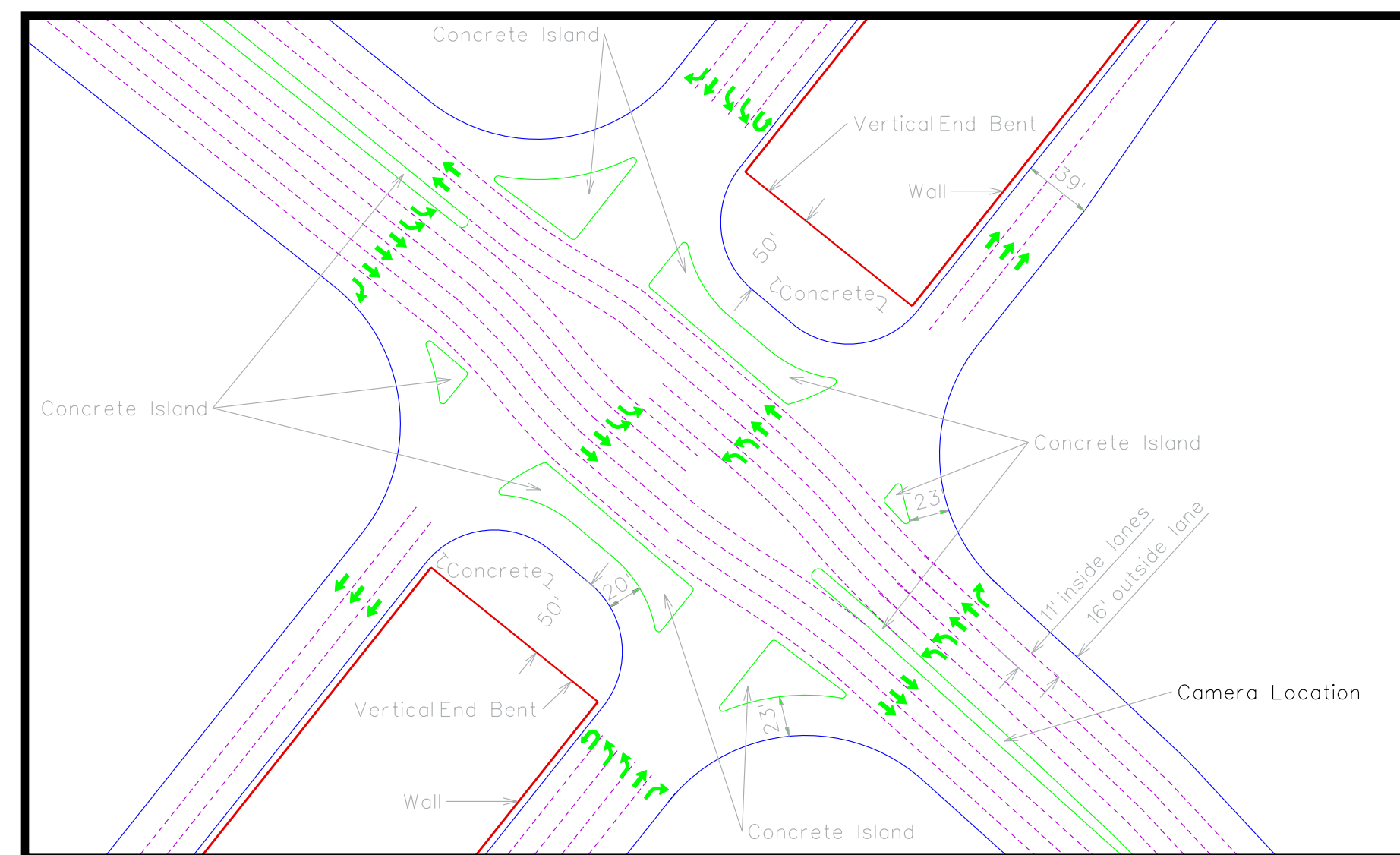
This schematic depicts all of the travel lanes and concrete islands of the proposed interchange, as well as the camera point of view for both the current and proposed views at right.
